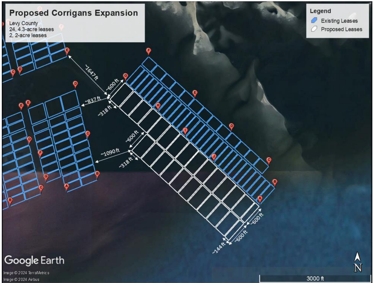
Figure 9. Proposed Lease parcels showing distances and recommended parcel schematic- 2-Acre and 4.3-Acre
