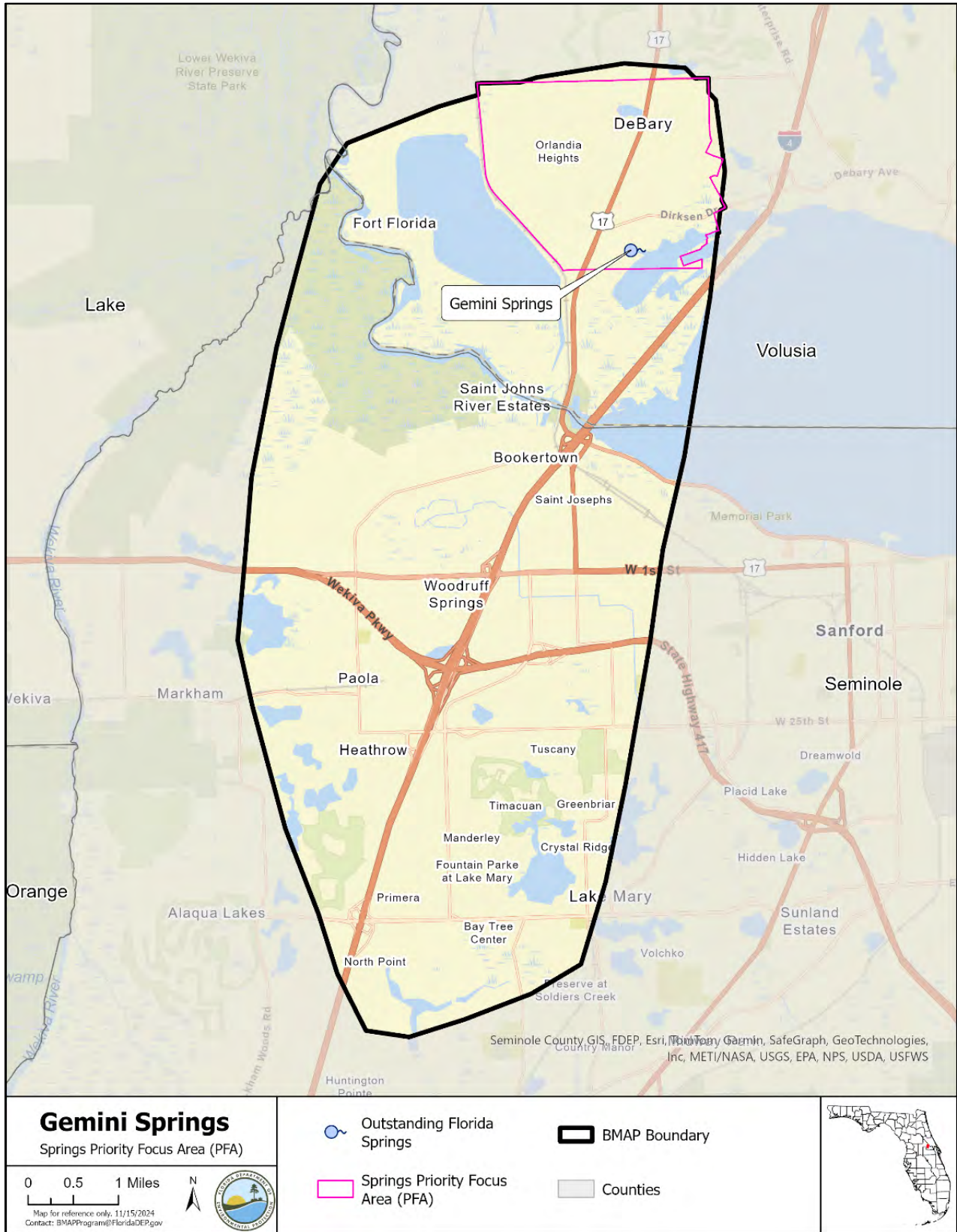
Figure ES-1. Gemini Springs BMAP and PFA boundaries
