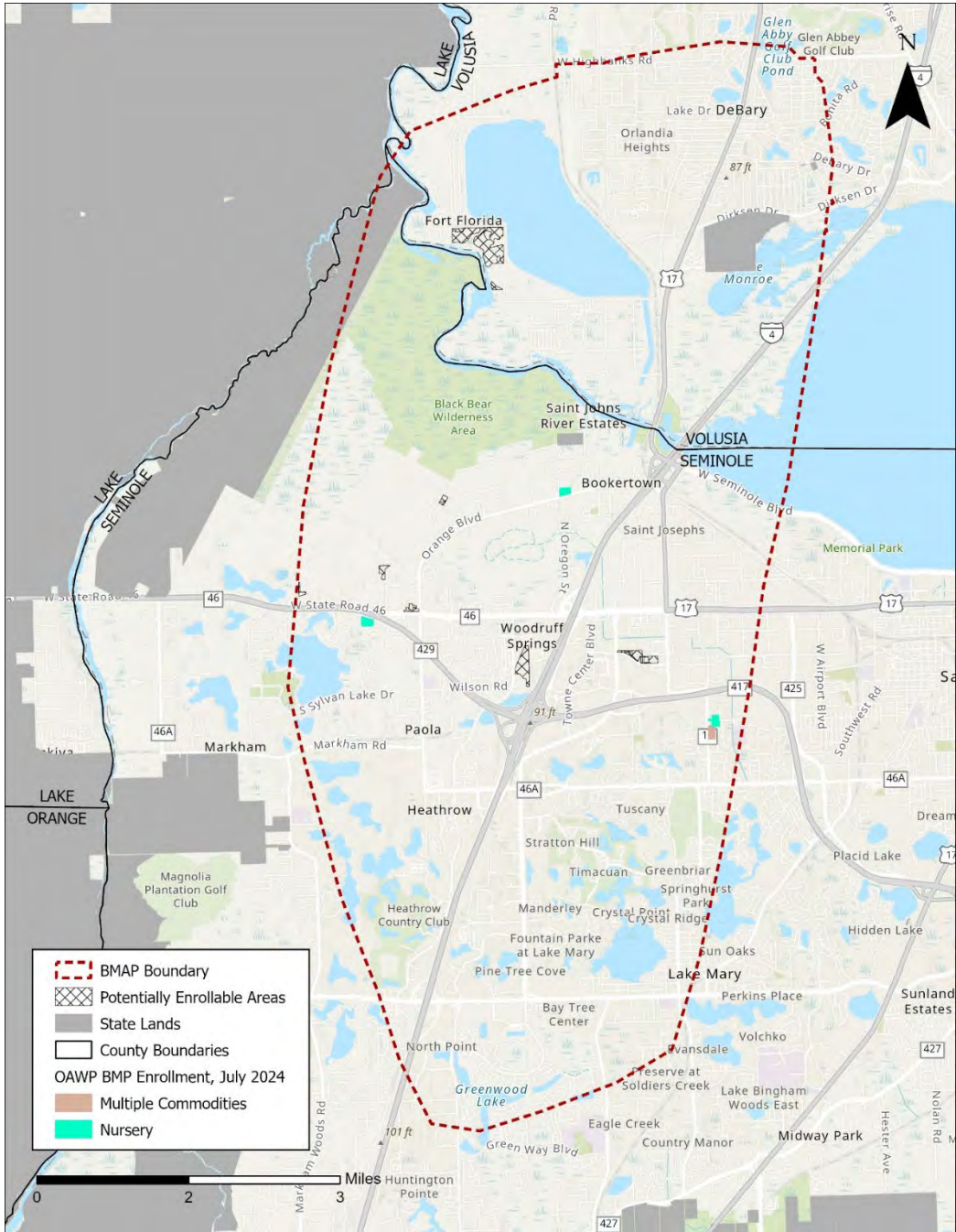
Figure H-2. Agricultural enrollment in the Gemini Springs BMAP
