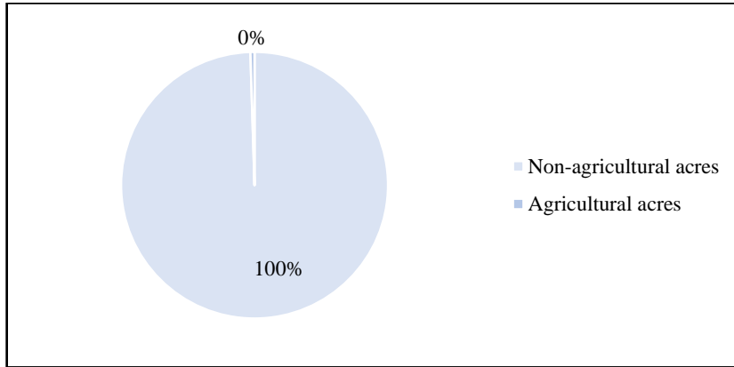
Figure H-1. Agricultural acres compared to non-agricultural acres in the BMAP area
