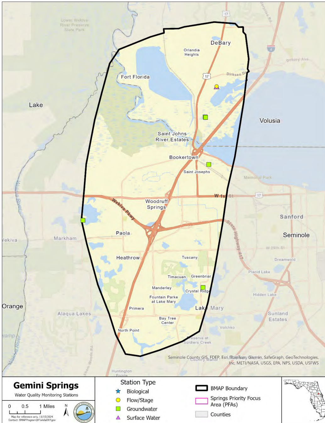
Figure 6. Monitoring stations in the Gemini Springs BMAP
