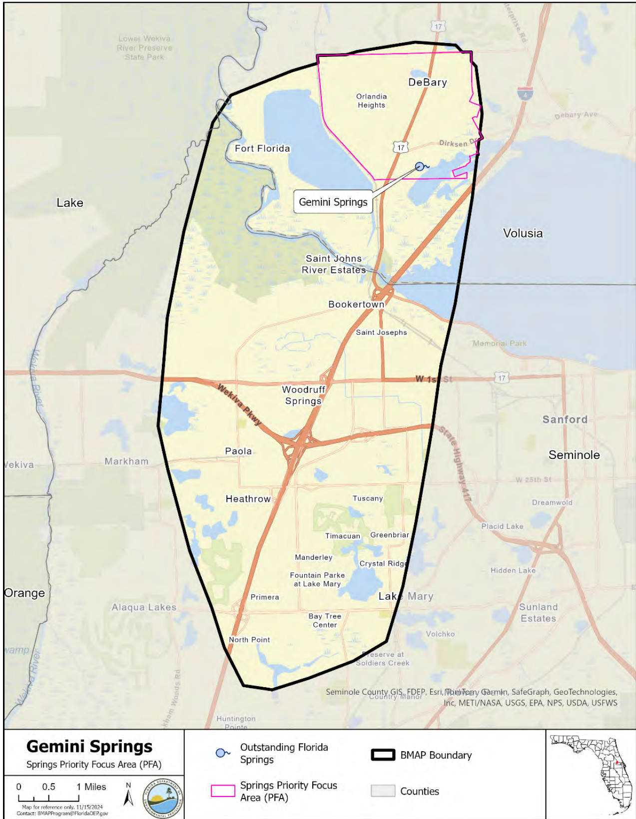
Figure 1. Gemini Springs BMAP and PFA boundaries
