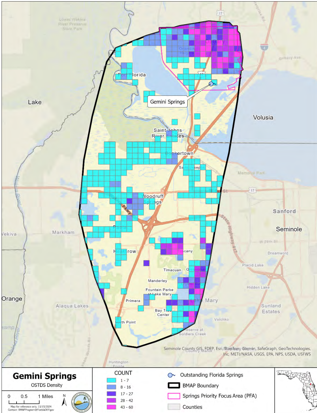
Figure E-1. Locations of OSTDS in the PFA in the Gemini Springs BMAP
