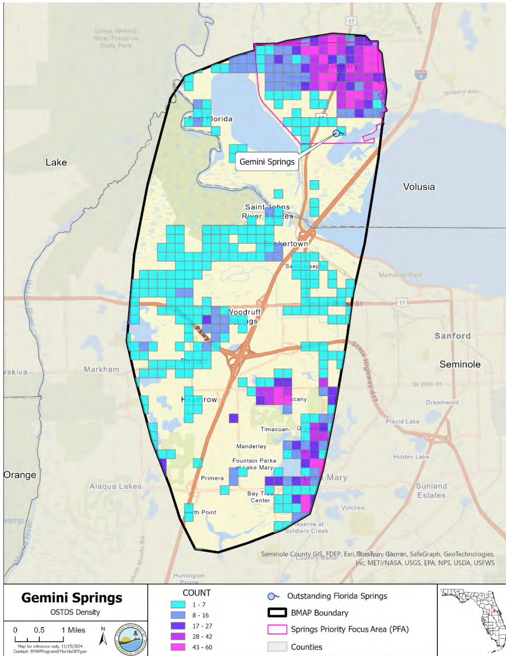
Figure 3. Estimated OSTDS location density in the Gemini Springs BMAP area and PFA
