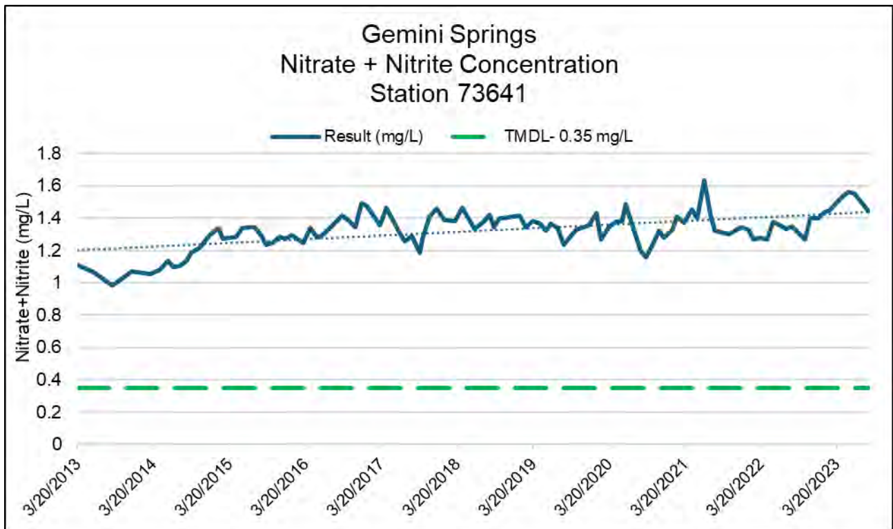
Figure 7. Nitrate plus nitrite concentration over time at station 73641
