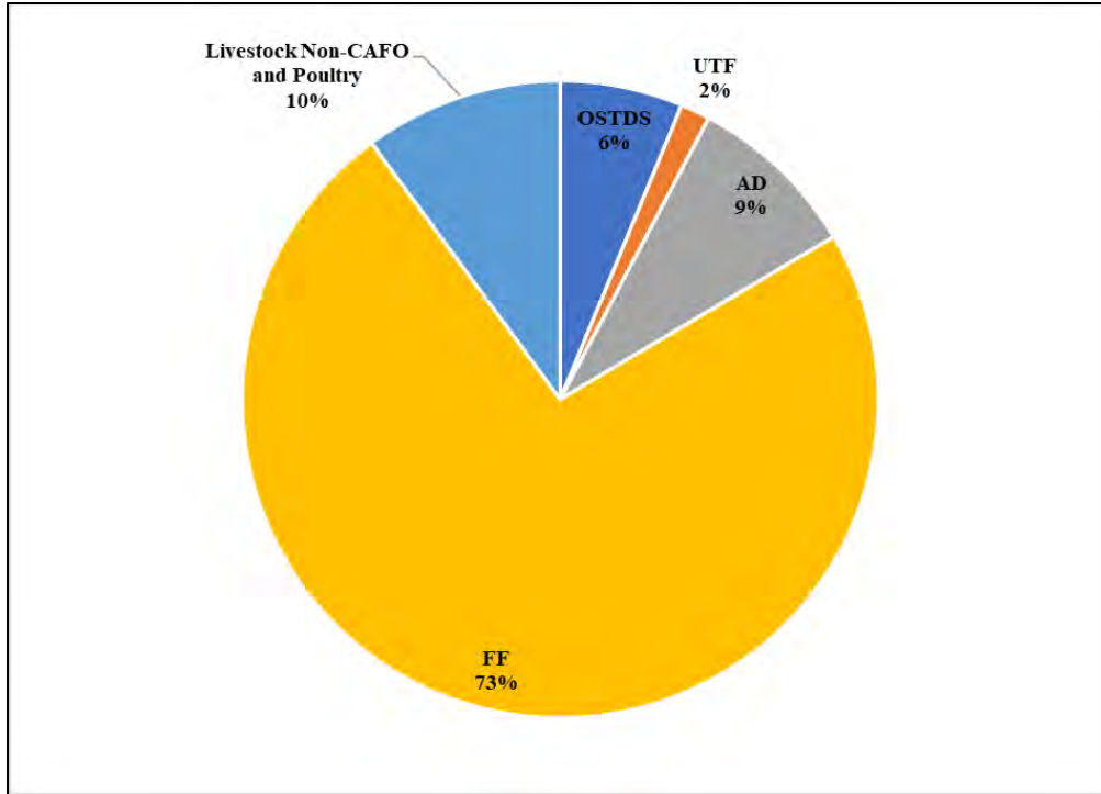
Figure 2. Loading to groundwater by source in the Madison Blue springshed area
