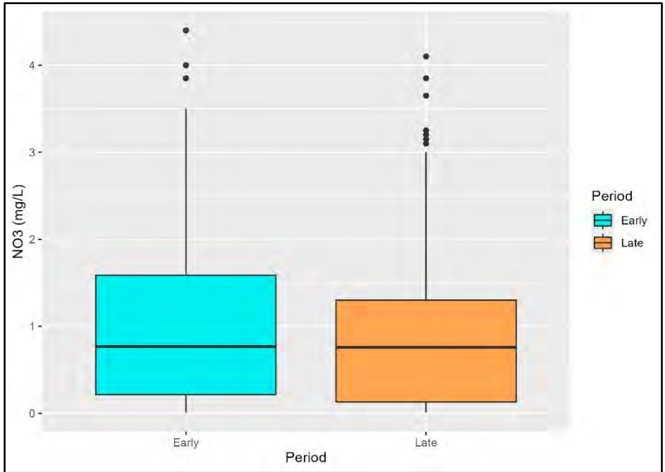
Figure 14. Lower Suwannee springshed nitrate concentrations of early and late periods with outliers
