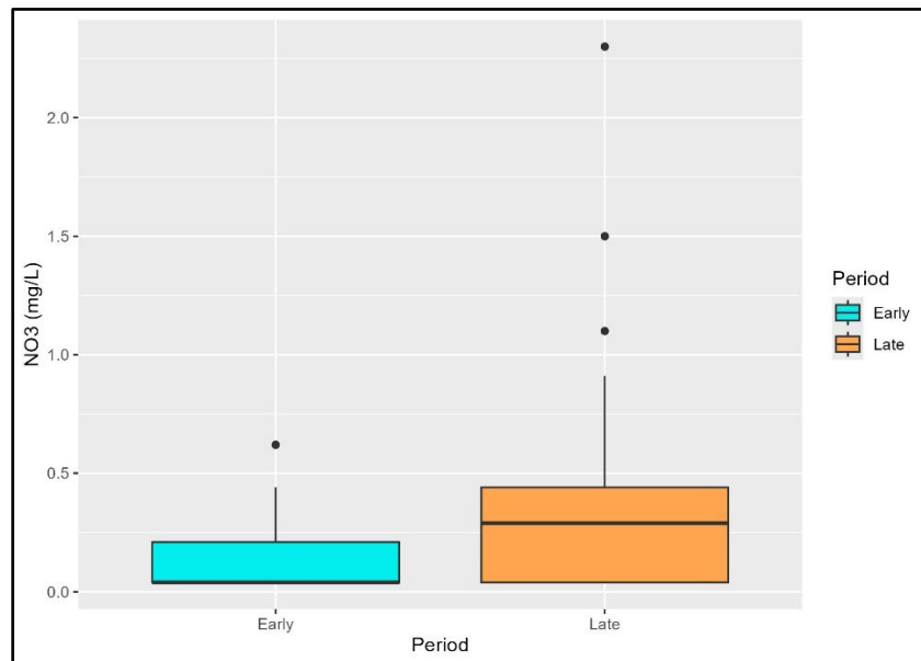
Figure 7. Crystal River/Kings Bay groundwater nitrate concentrations of early and late periods with outliers
