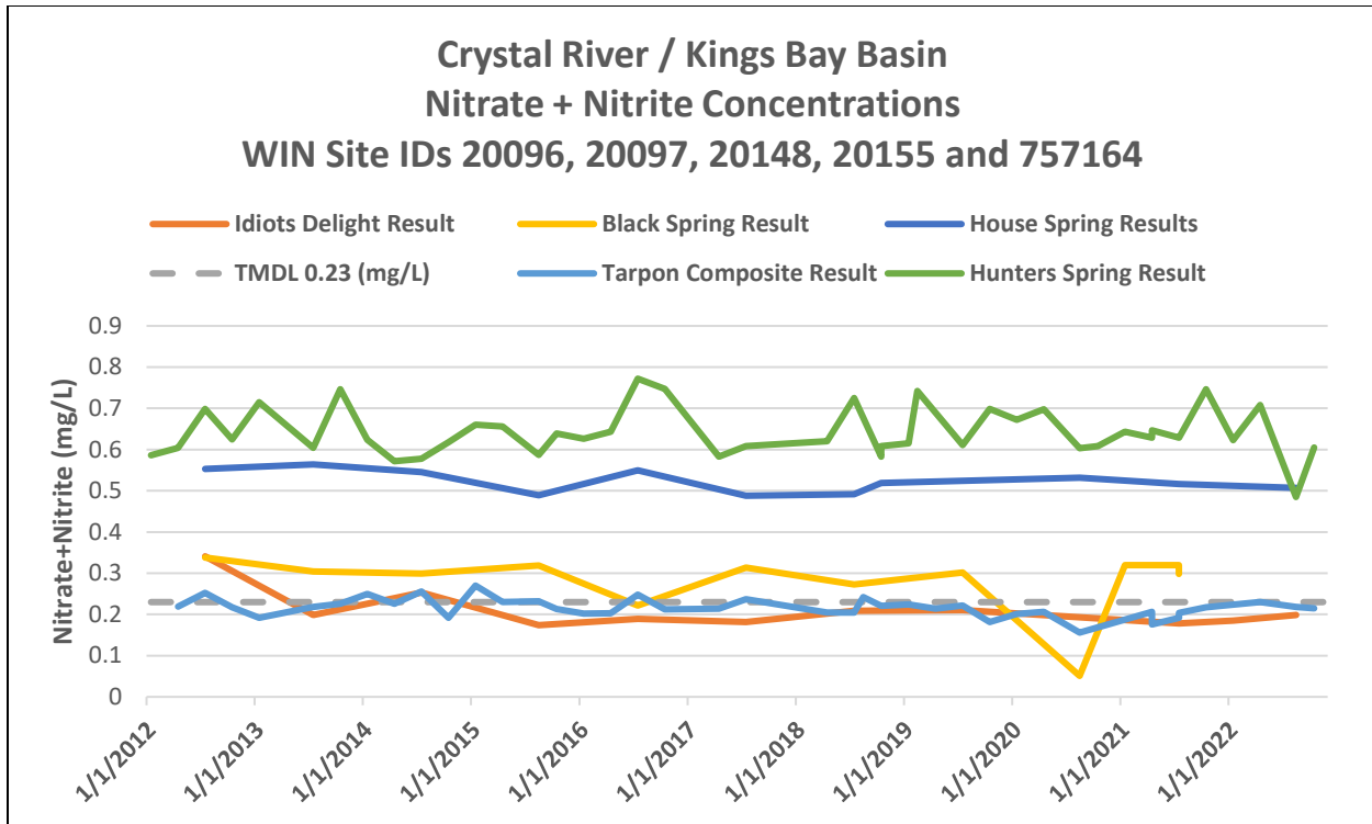
Figure 6. Nitrate plus nitrite concentration over time at stations 20096, 20097, 20148, 20155 and 757164
