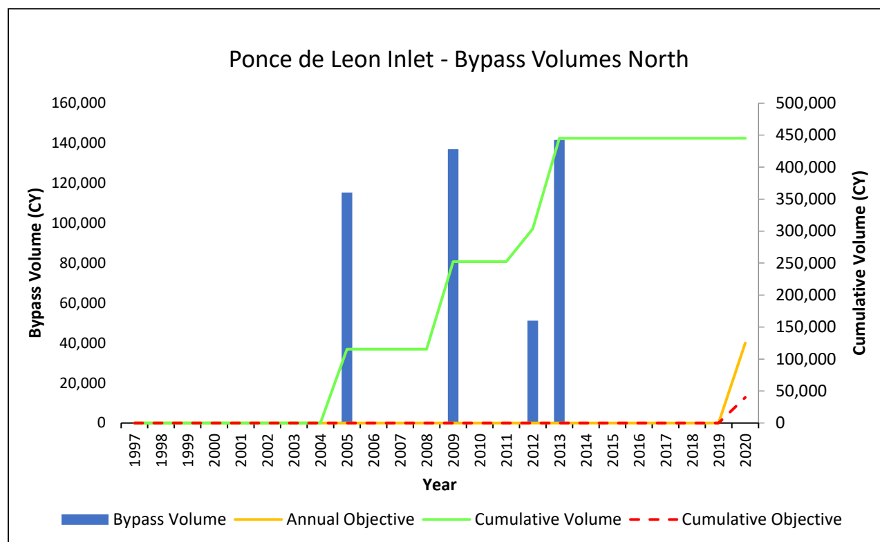
Figure 5: Ponce de Leon Inlet bypass volume, annual objective, cumulative volume and cumulative objective.
