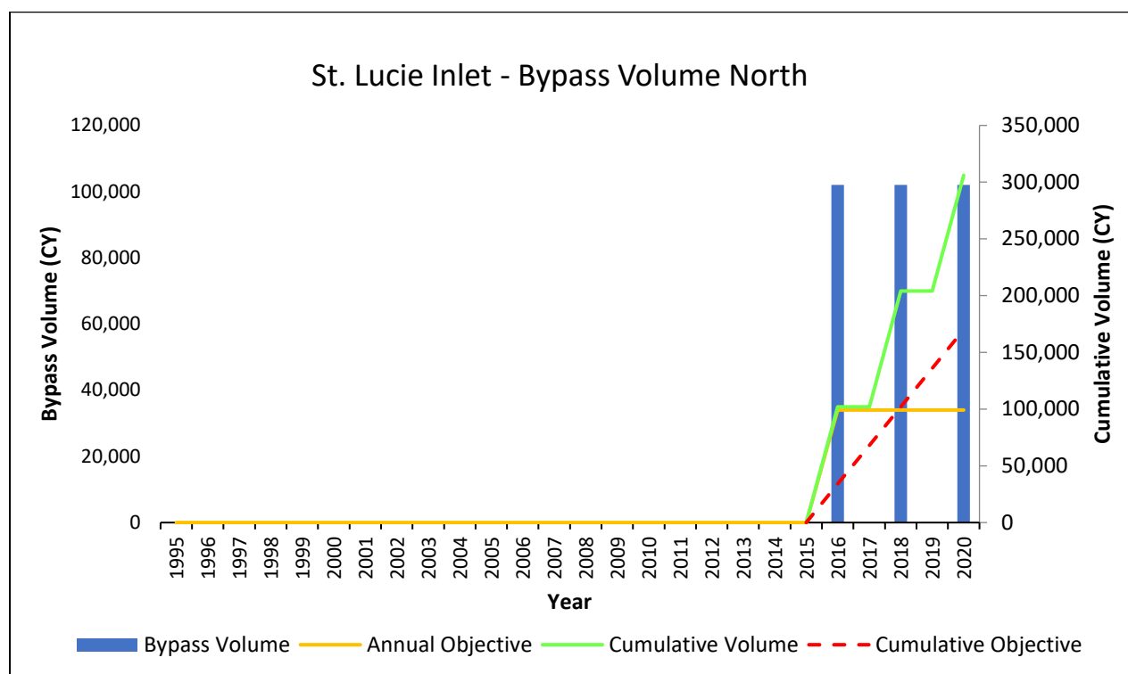
Figure 11: St. Lucie Inlet bypass volume, annual objective, cumulative volume and cumulative objective.
