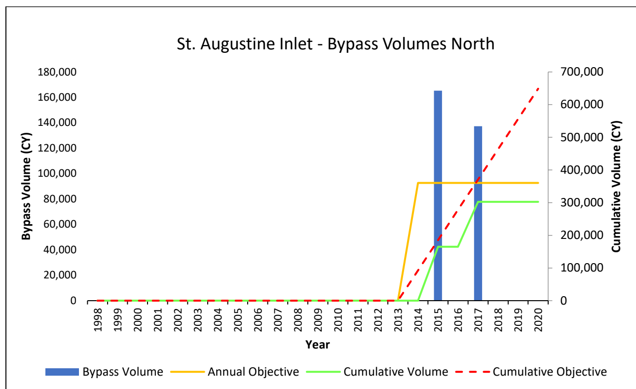
Figure 3: St. Augustine Inlet bypass volume, annual objective, cumulative volume and cumulative objective.
