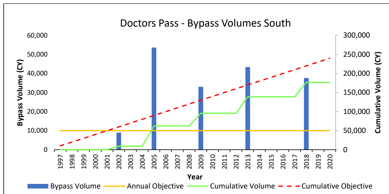
Figure 34: Doctors Pass bypass volume, annual objective, cumulative volume and cumulative objective.
