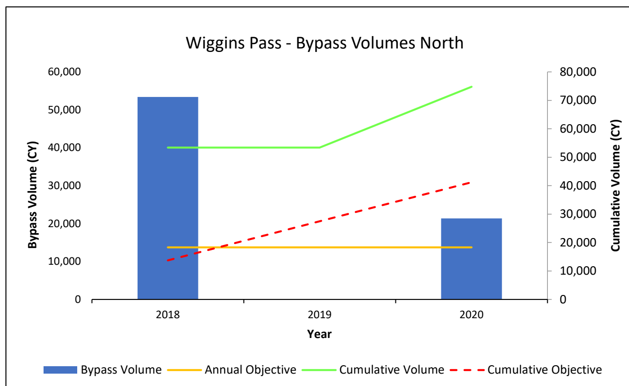
Figure 32: Wiggins Pass bypass volume, annual objective, cumulative volume and cumulative objective.
