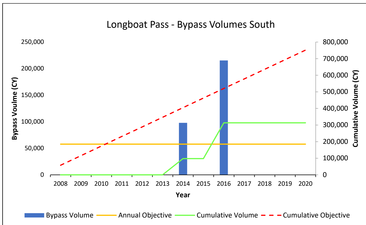
Figure 28: Longboat Pass bypass volume, annual objective, cumulative volume and cumulative objective.
