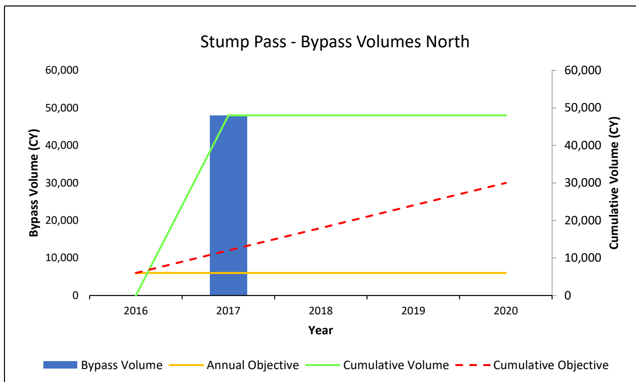
Figure 30: Stump Pass bypass volume, annual objective, cumulative volume and cumulative objective.
