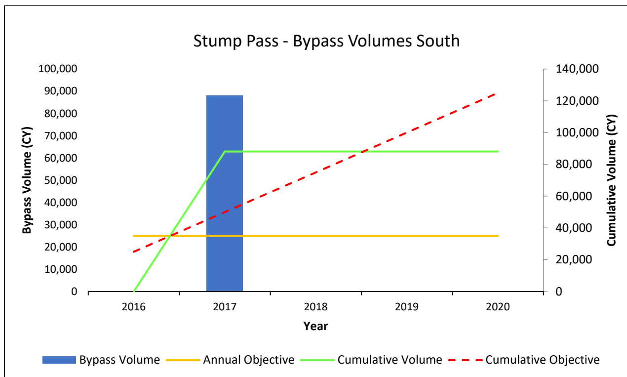
Figure 31: Stump Pass bypass volume, annual objective, cumulative volume and cumulative objective.
