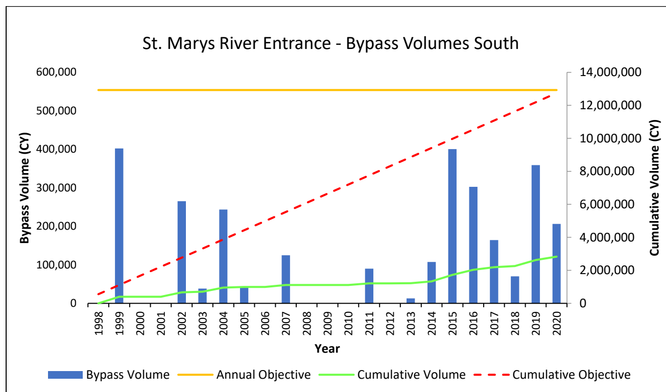
Figure 2: St. Marys River Entrance bypass volume, annual objective, cumulative volume and cumulative objective.
