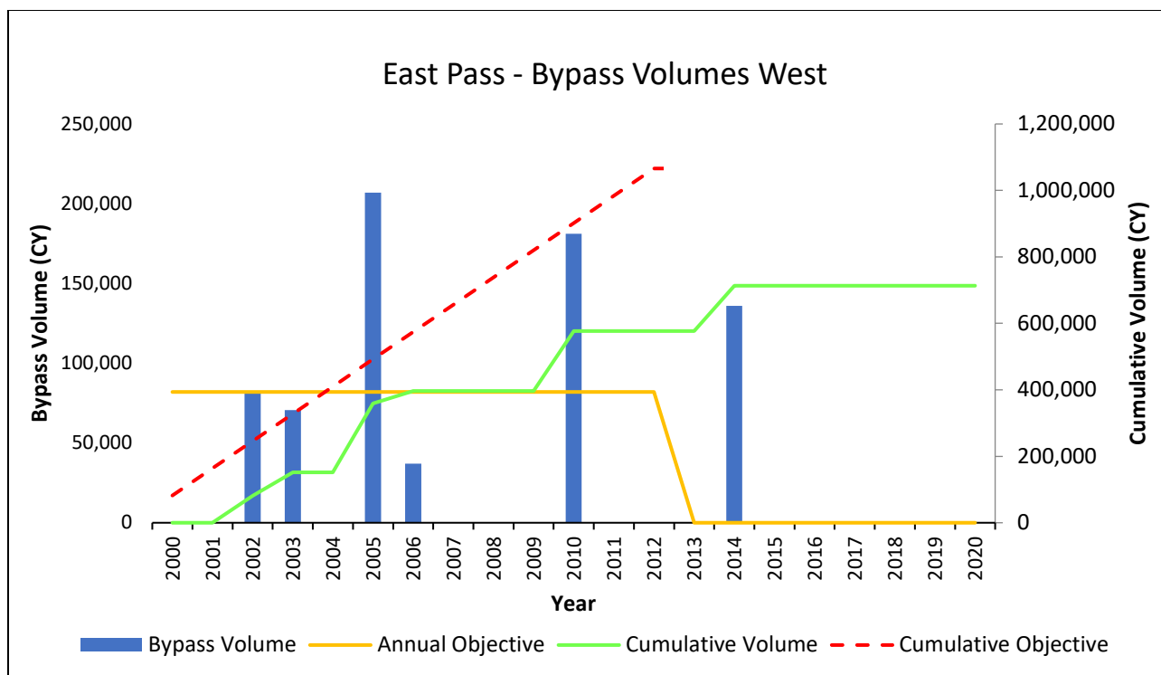
Figure 23: East Pass bypass volume, annual objective, cumulative volume and cumulative objective.
