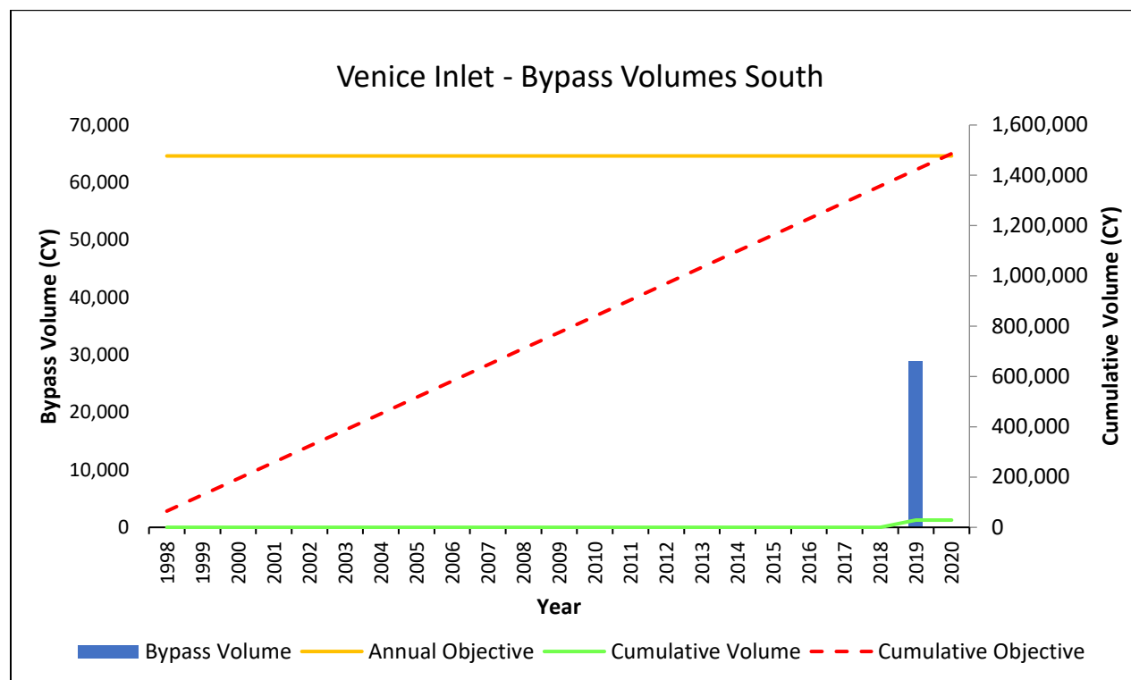
Figure 29: Venice Inlet bypass volume, annual objective, cumulative volume and cumulative objective.
