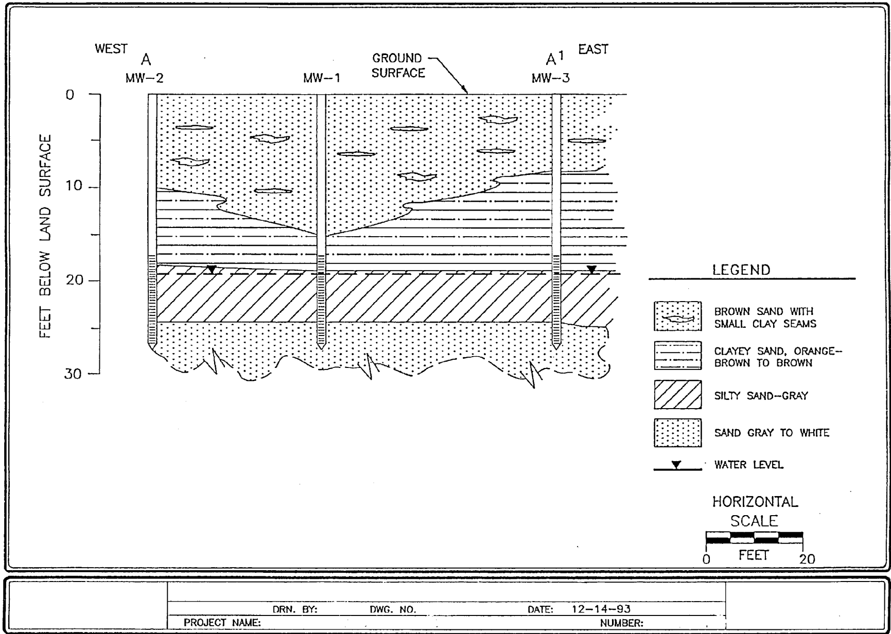
FIGURE 5-7. GEOLOGIC CROSS SECTION A-A 1
