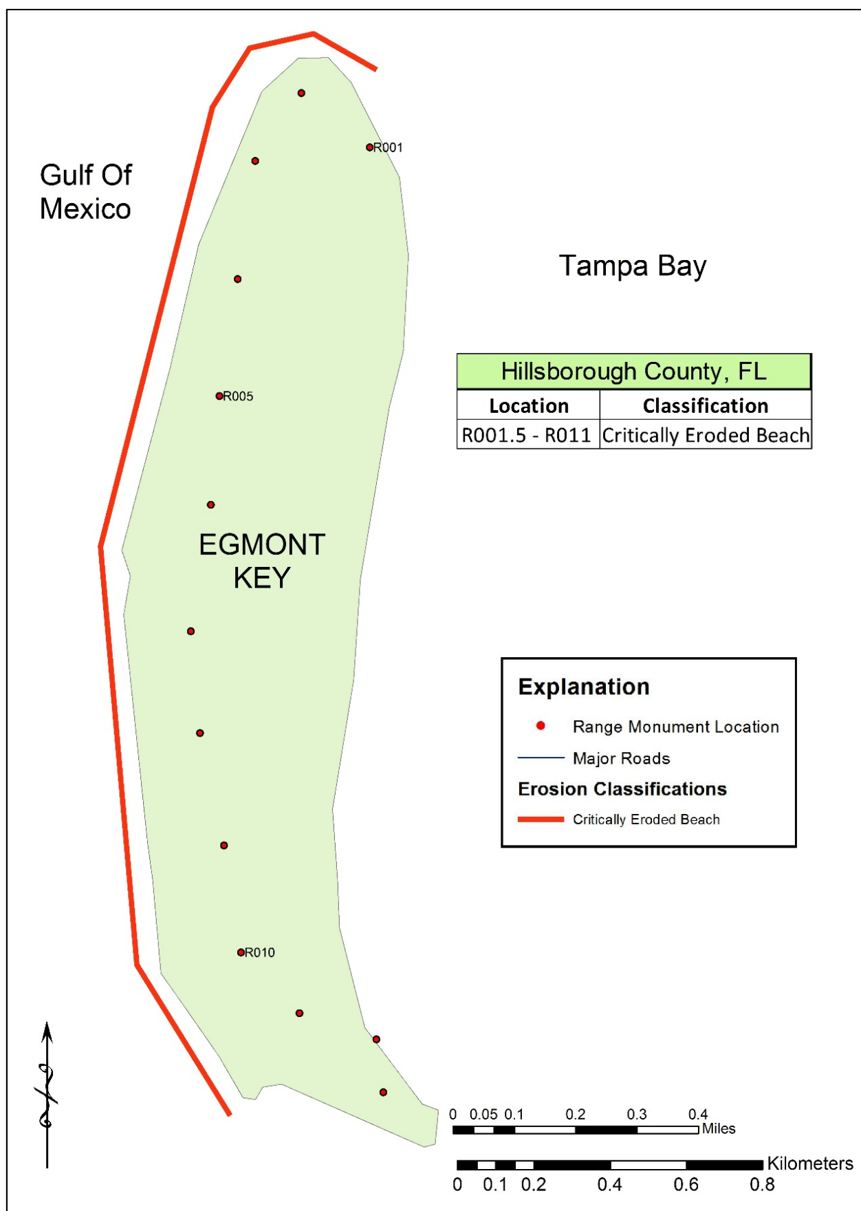
Figure 25. Critically eroded shoreline within Hillsborough County.
