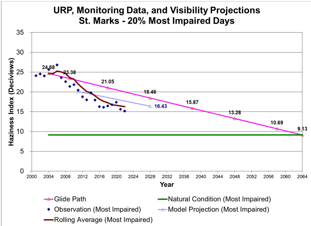
Figure 4-5. St. Marks National Wilderness Area Visibility Impairment on the 20% Most Impaired Days, Glide Path, and 2028 RPG
