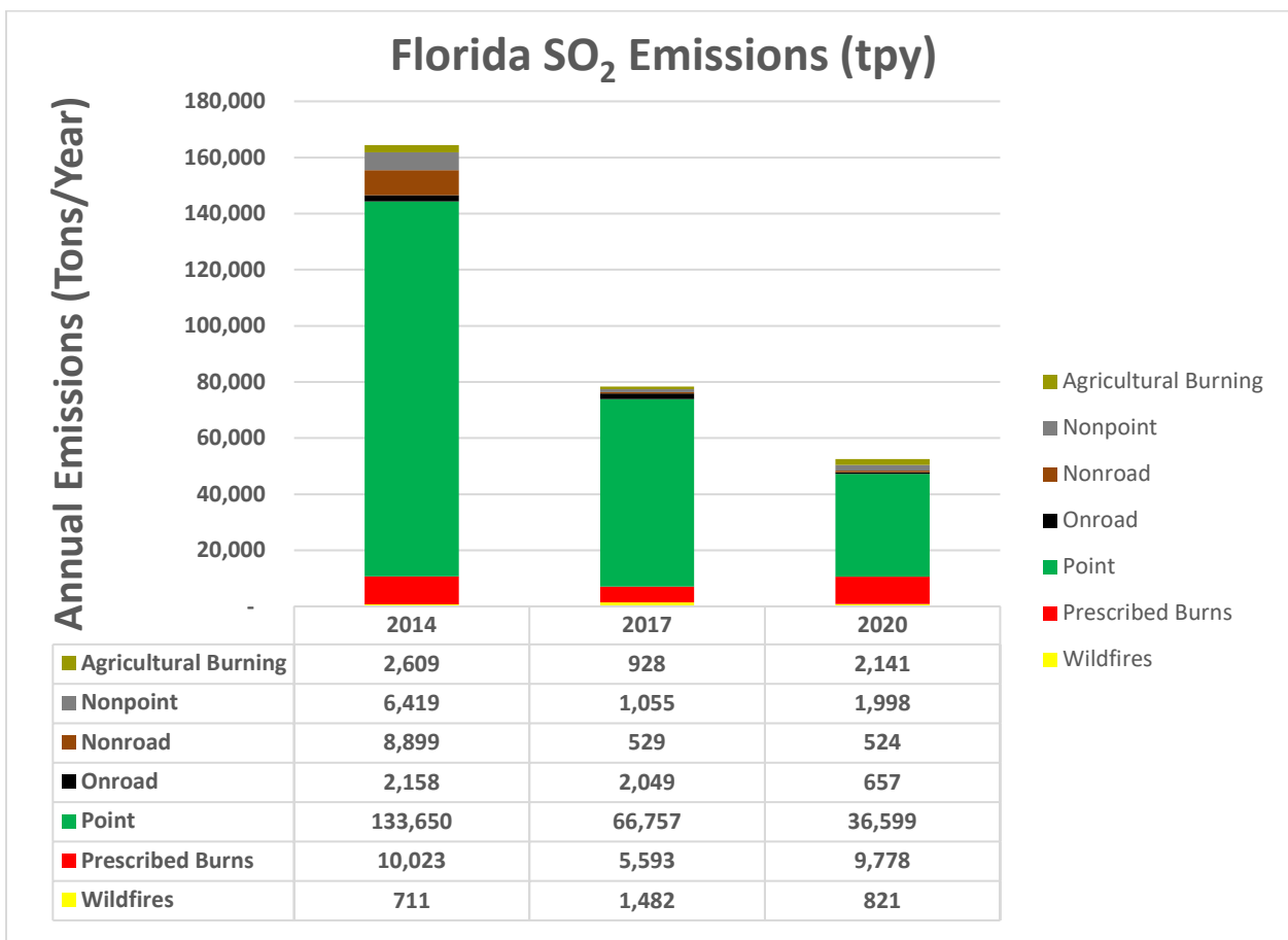
Figure 5-3. Florida SO 2 Emissions (in tons) by Category
