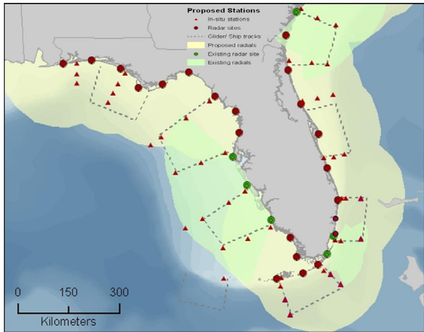
Figure 4: A schematic of an ideal Florida COOS offshore coastal ocean observational base network array based on unlimited funds and assuming no existing infrastructure or long-term observations (not shown: satellite remote sensing and coastal stations). (Adapted from SEACOOS).
