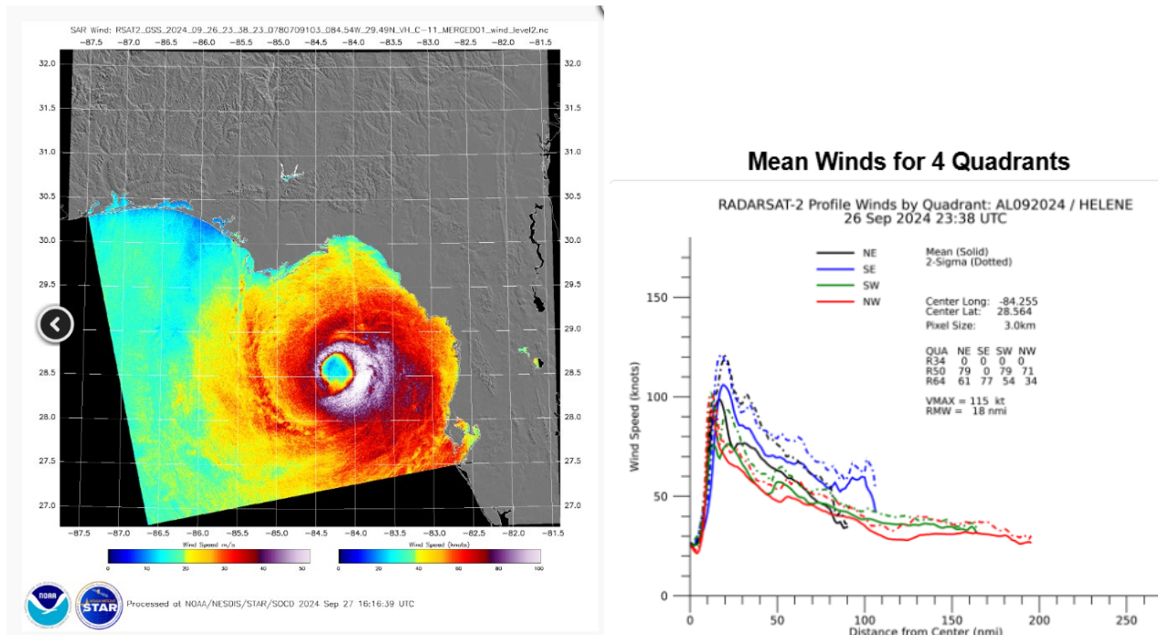
Figure 5. Synthetic Aperture Radar (SAR) imagery showing the spatial distribution of Hurricane Helene’s wind field impacting Florida’s Big Bend Coast (NOAA).
