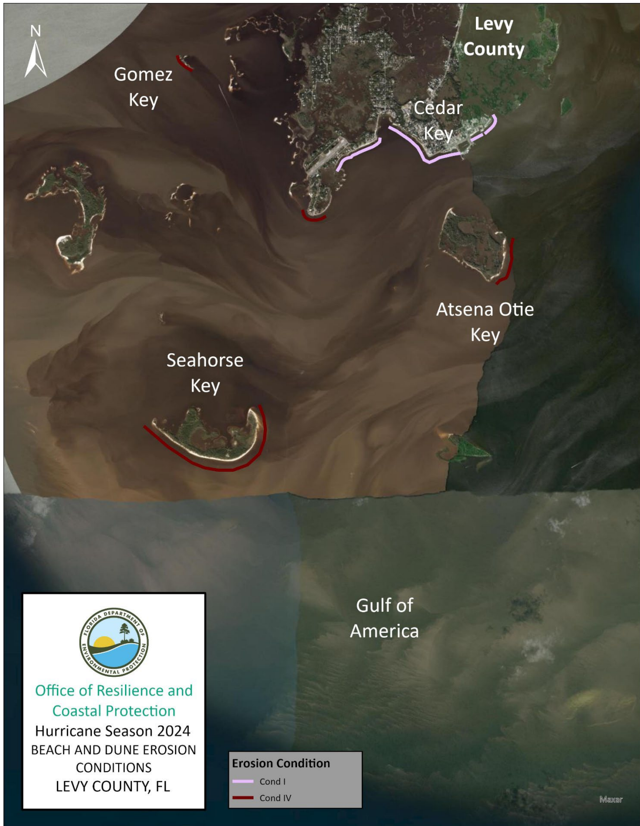
Figure 51. Southern Levy County beach and dune erosion conditions from Hurricane Helene.
