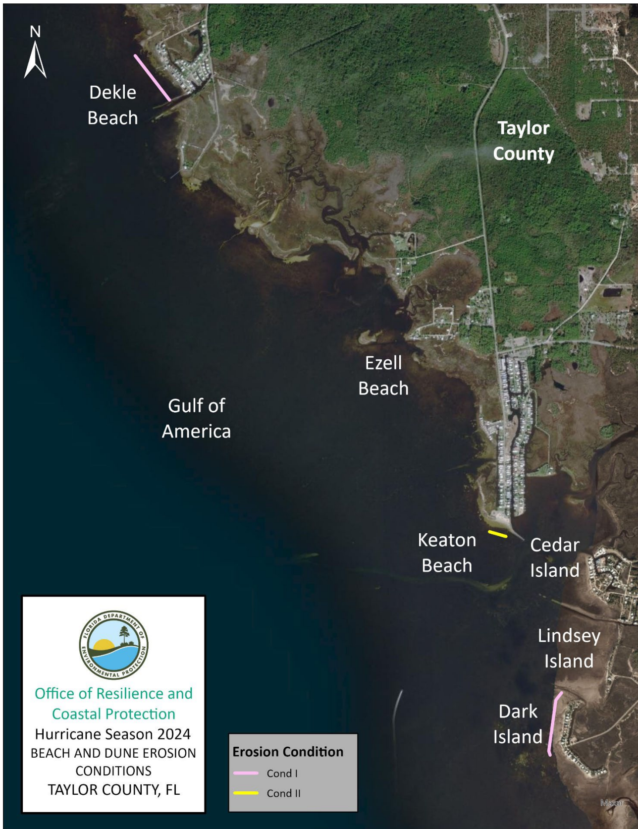
Figure 13. Taylor County beach and dune erosion conditions from Hurricane Helene.
