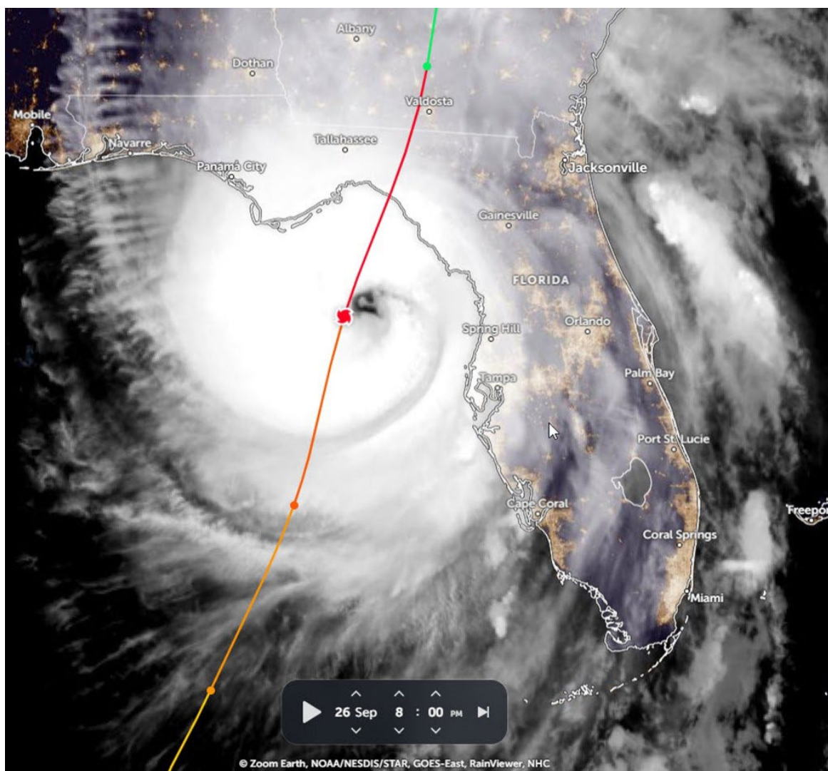
Figure 4. Hurricane Helene track overlaid on satellite imagery (source: Zoom Earth).
