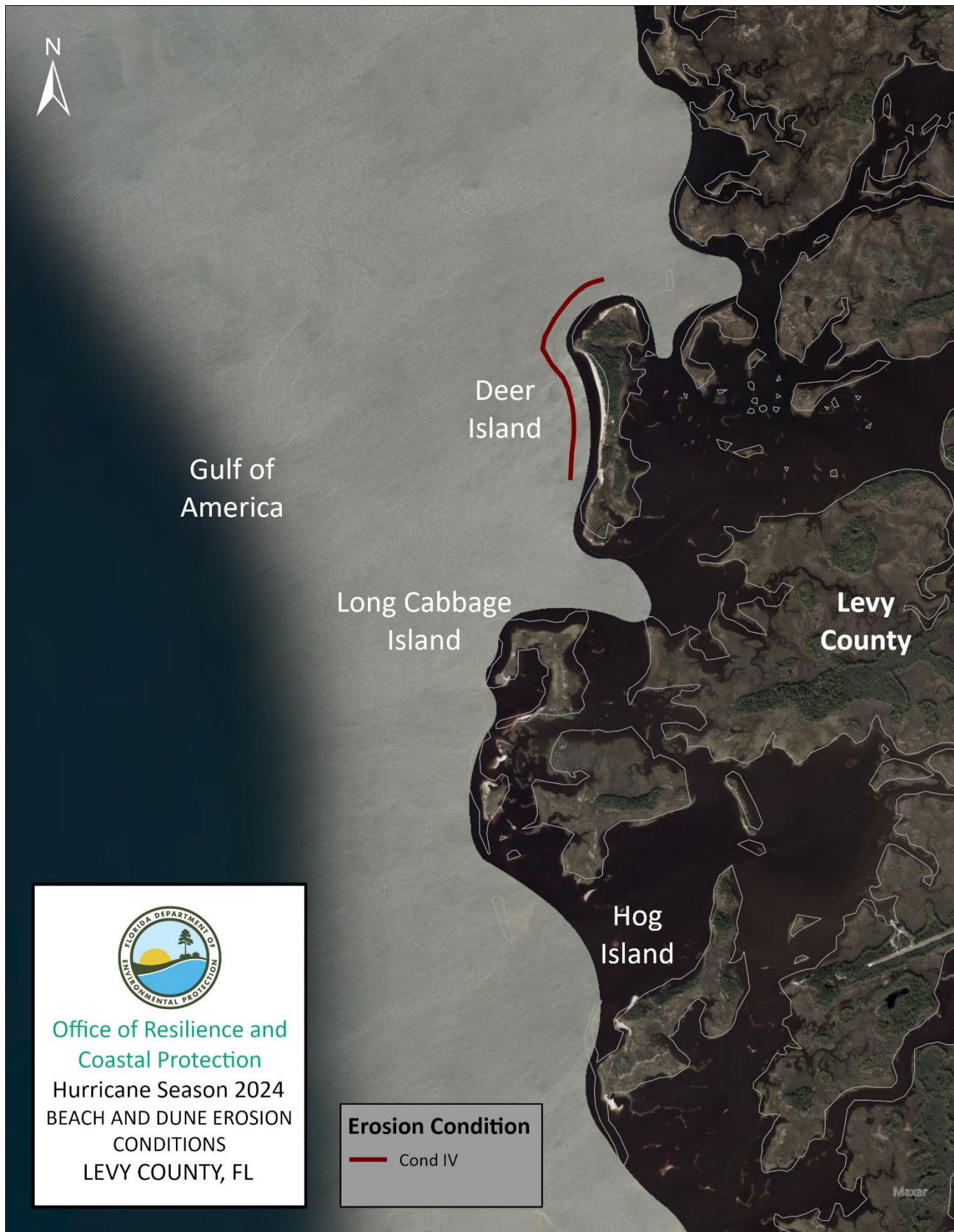
Figure 50. Northern Levy County beach and dune erosion conditions from Hurricane Helene.
