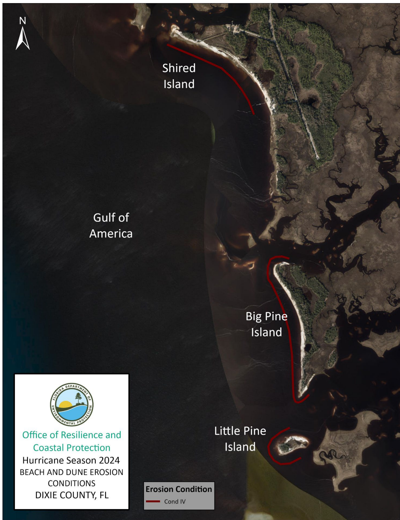
Figure 30. Southern Dixie County beach and dune erosion conditions from Hurricane Helene.
