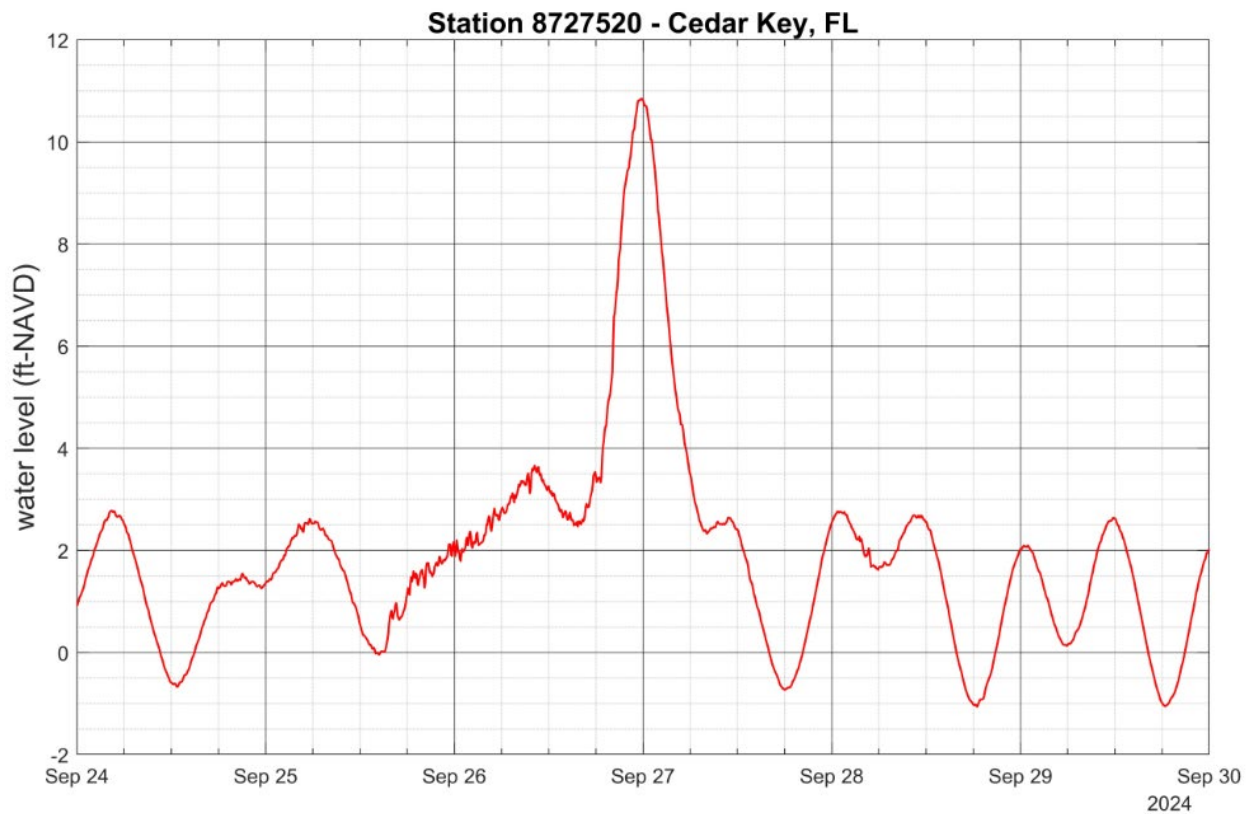
Figure 9. Water level elevations at Cedar Key, FL (NOAA).
