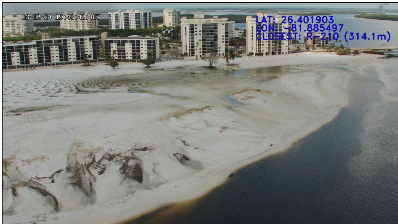
Figure 136. Major beach and dune erosion (condition IV) due to Helene and Milton at south end of Estero Island (Ft. Myers Beach) near R-210.
