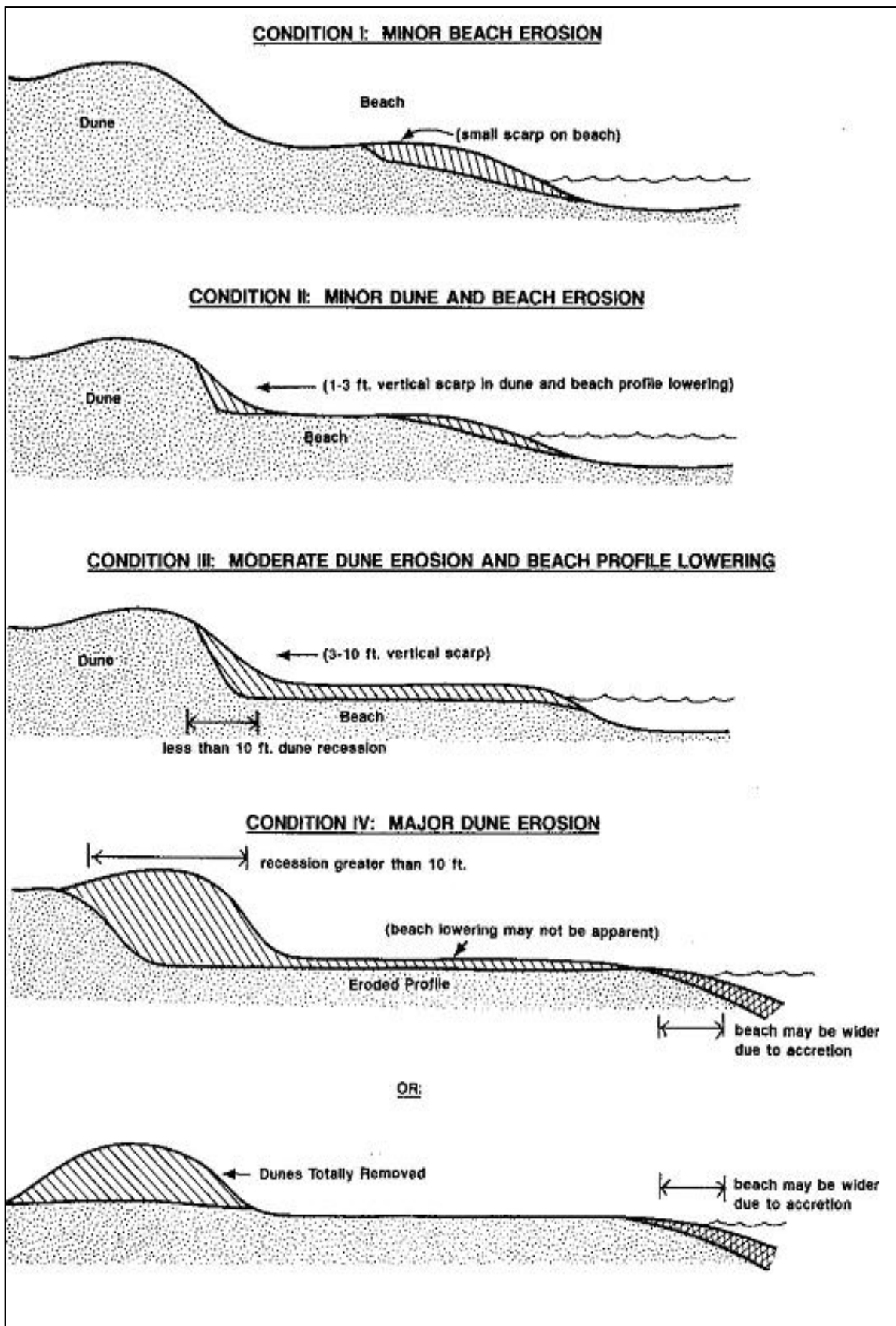
Figure 10. Beach Erosion Conditions I to IV.
