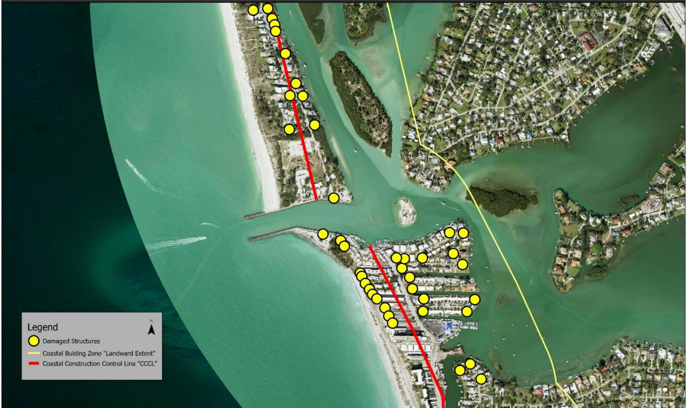
Figure 1. A snapshot of DEP data points collected at Casey Key in Sarasota County after Hurricane Helene within the coastal building zone that goes landward to the yellow line.
