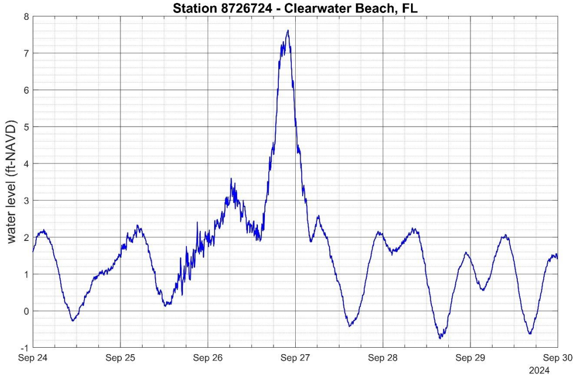
Figure 3. Water level elevations at Clearwater Beach, FL (Data Source: NOAA).
