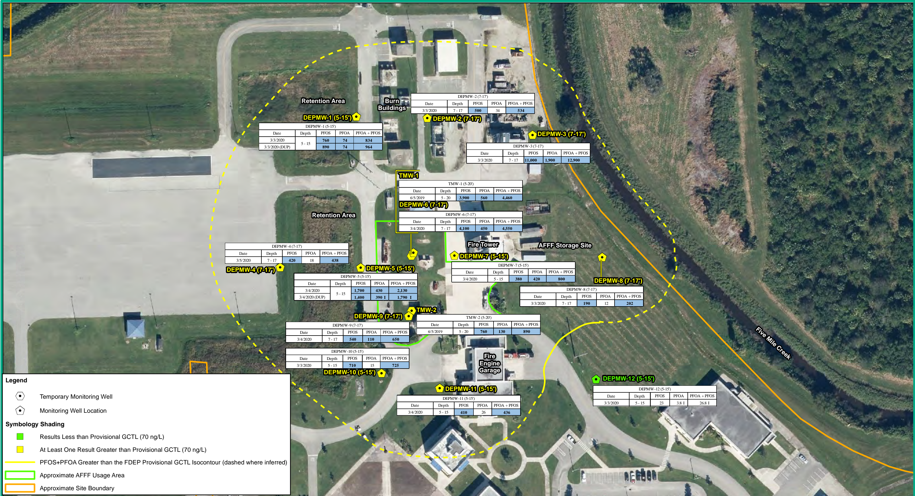
Figure 20 Summary of Analytical Results in Groundwater from 5 to 17 ft BLS Indian River State College 4600 Kirby Loop Road Fort Pierce, St. Lucie County, Florida
