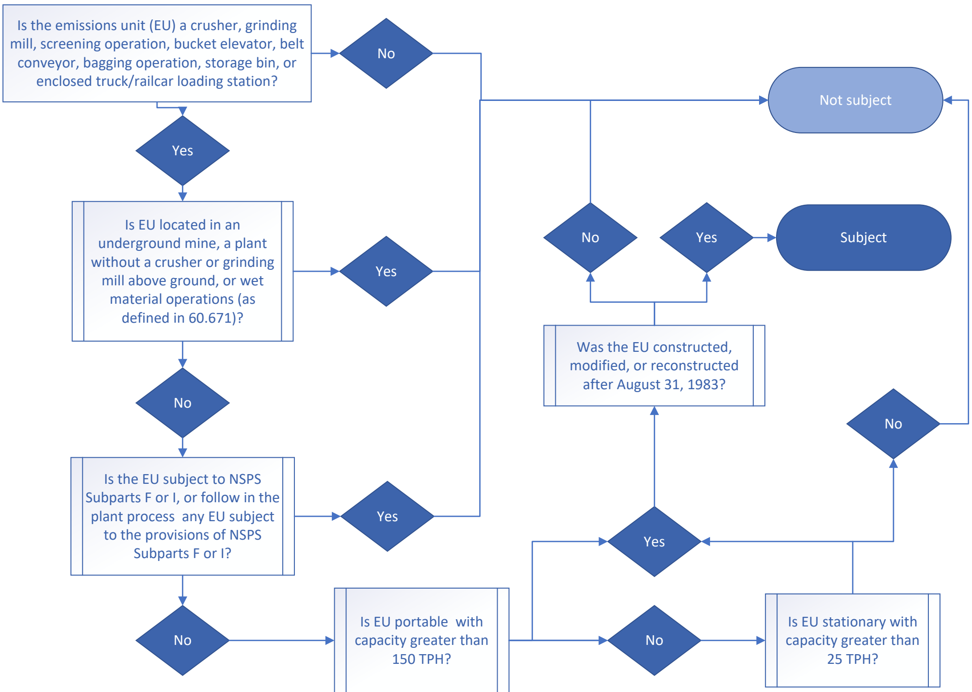
NSPS Subpart 000 Applicability Flow Chart
