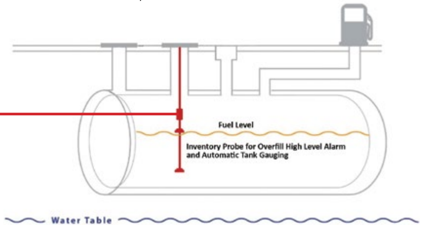
Overfill High Level Alarm System Using Automatic Tank Gauging
