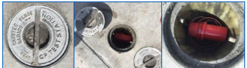
CP Test Stations
