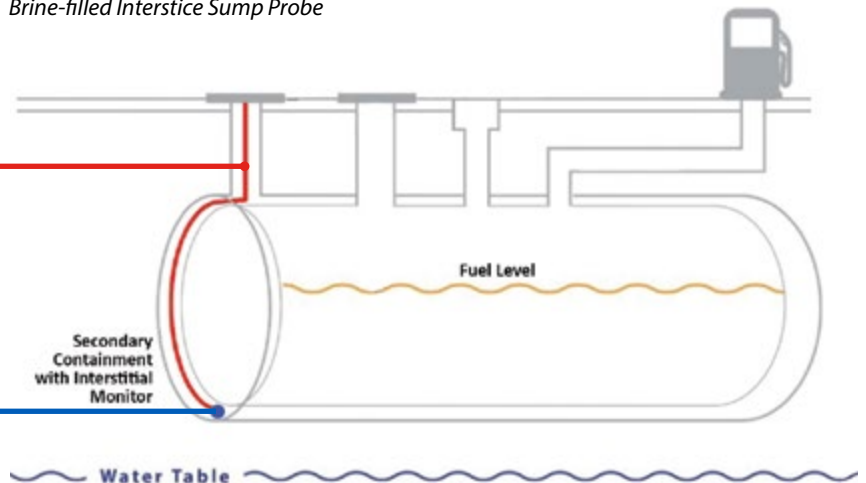
Dry Secondary Containment with Interstitial Sensor/Probe
