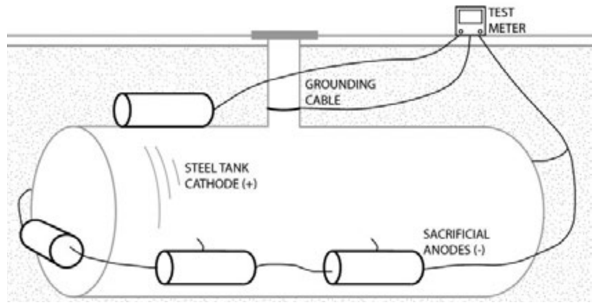
Galvanic CP System with Sacrificial Anodes Attached
