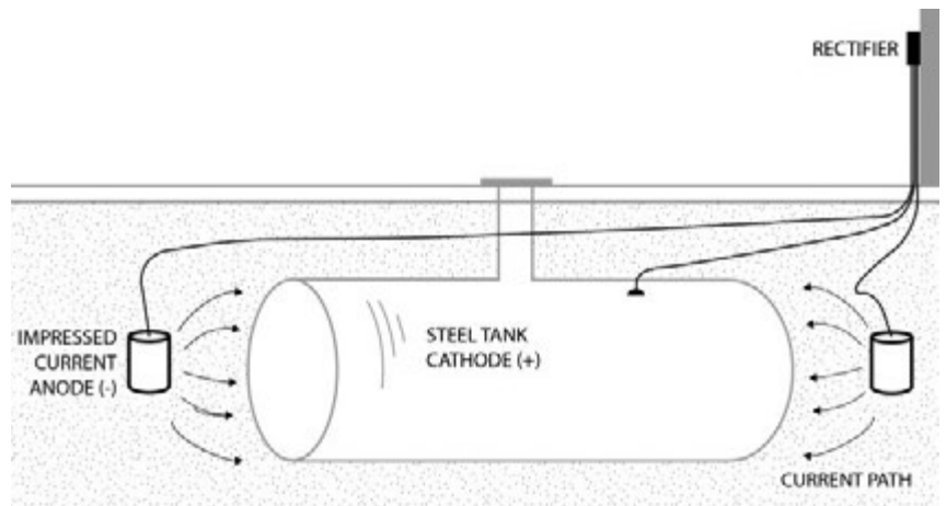
Impressed Current CP System
