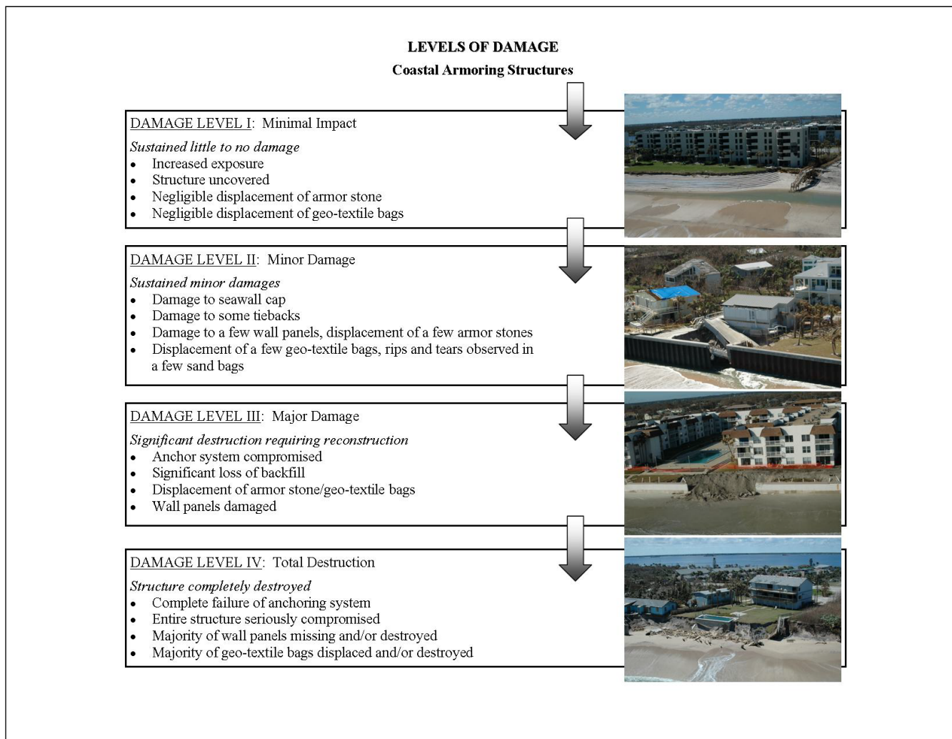
Figure 117. DEP’s Coastal Engineering graphic describing the levels of damage (I – IV) to coastal armoring structures, including seawalls and revetments.
