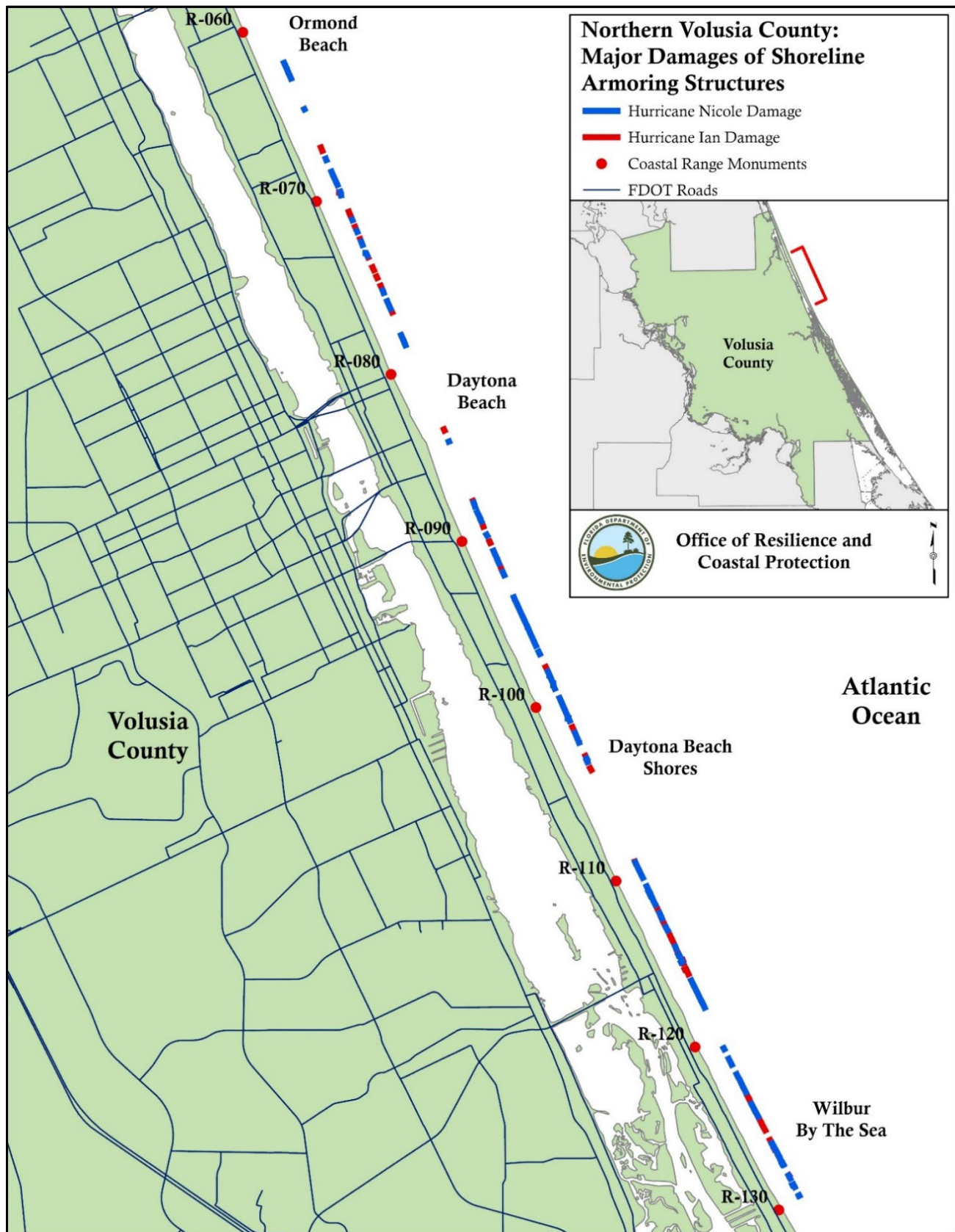
Figure 96. Major damages to armoring after Hurricanes Ian and Nicole in northern Volusia County. Note: see Appendix A or Figure 117 that describes the different damage levels to coastal armoring structures.
