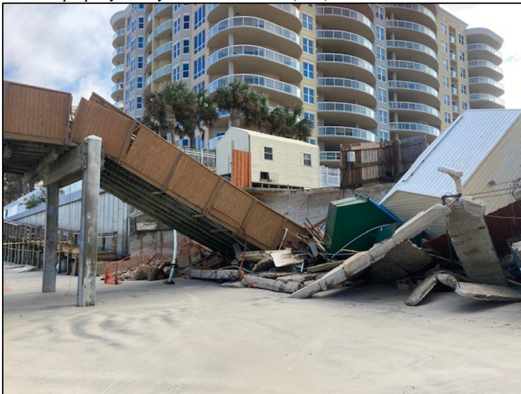
Figure 84. Multiple failures: landward section of Sun Glow Pier, seawall destroyed, building and parking lot destroyed (R118).
