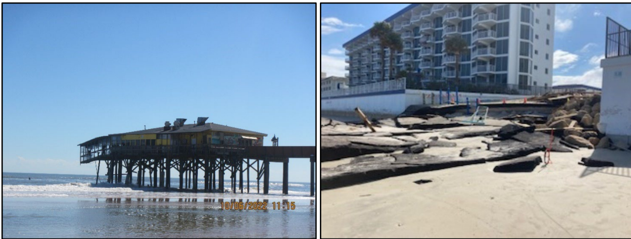
Figure 78. Sun Glow Fishing Pier destroyed (left, R118); Demotte Ave. beach ramp destroyed (right, R116).
