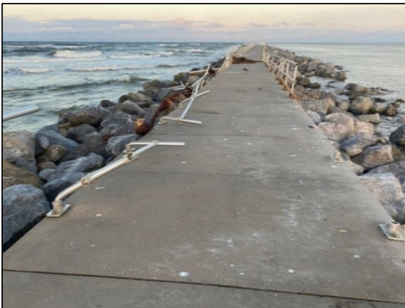
Figure 94. Damaged north jetty fishing pier at Ponce de Leon Inlet (R148).
