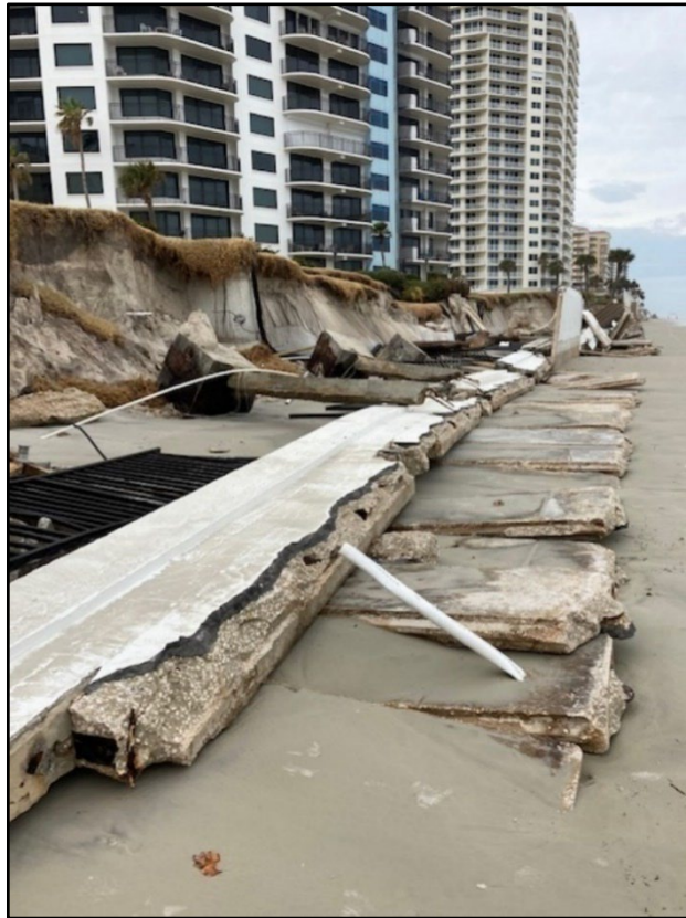
Figure 91. Catastrophic seawall failure threatens buildings in Daytona Beach (R75).
