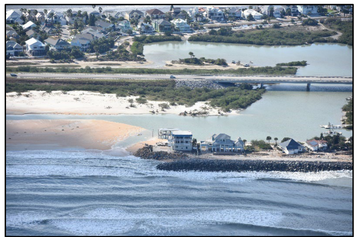
Figure 60. Coastal barrier breaches at Summer Haven at R204.9 (left) and R200 (right). Aerial oblique photos taken by the Civil Air Patrol on November 12, 2022.
