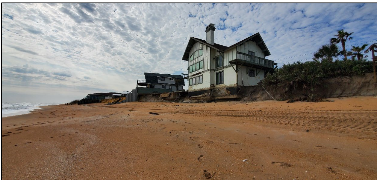
Figure 66. Single-family dwelling with first floor damage and major pool damage in Beverly Beach (R-53).
