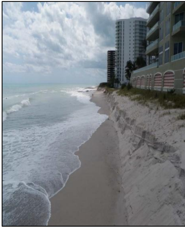
Figure 6. Condition III or Moderate Dune Erosion.
