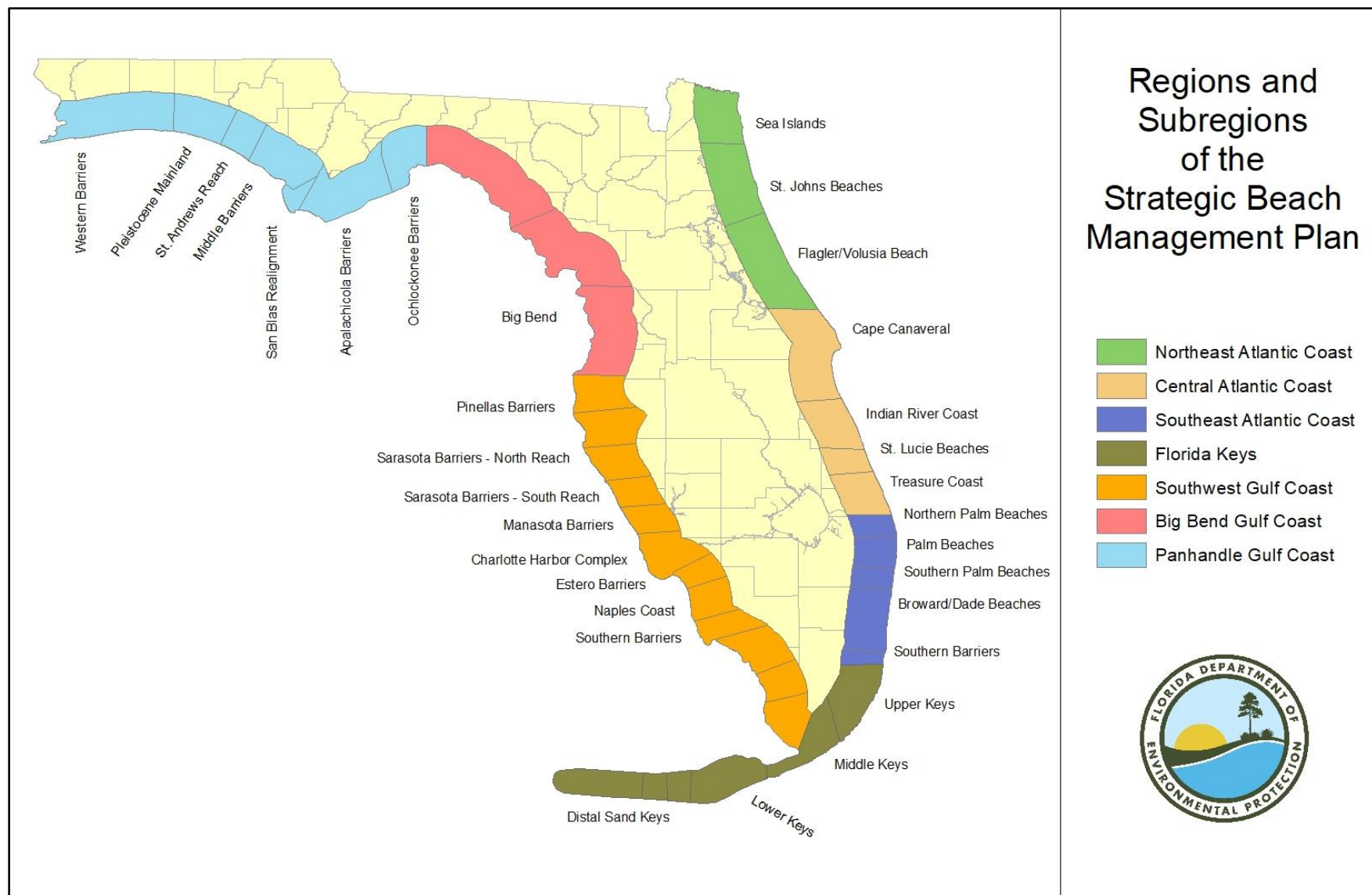
Figure 2. Map of the statewide SBMP's regions and subregions. View an interactive map .
