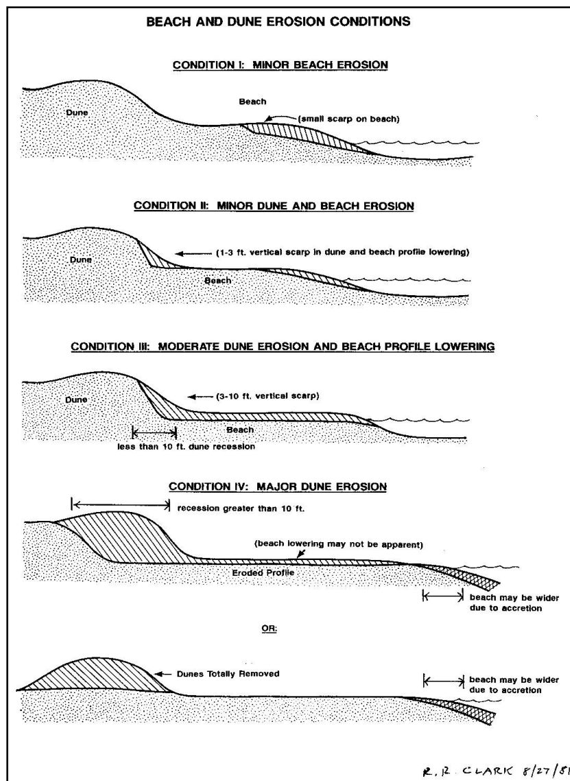
Figure 3. Graphic illustrating beach and dune erosion conditions.
