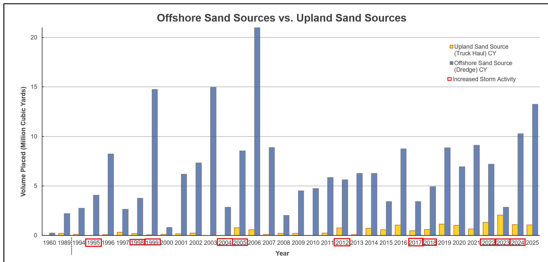
Figure 16. The bar graph compares the volumes of offshore sand (dredged) to upland sand (truck hauled) used in beach nourishment or dune restoration projects (excluding placement of sand in nearshore areas) between 1960 through 2025.
