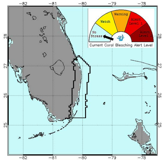
Figure 1. NOAA Coral Reef Watch Bleaching Alert Area for November 13 2017. https://coralreefwatch.noaa.gov/vs/gauges/southeast_florida.php
