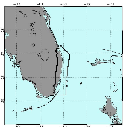
Figure 2 (left). NOAA CRW Hotspots for November 13, 2017. http://coralreefwatch.noaa.gov/satellite/bleaching5km/index.php
