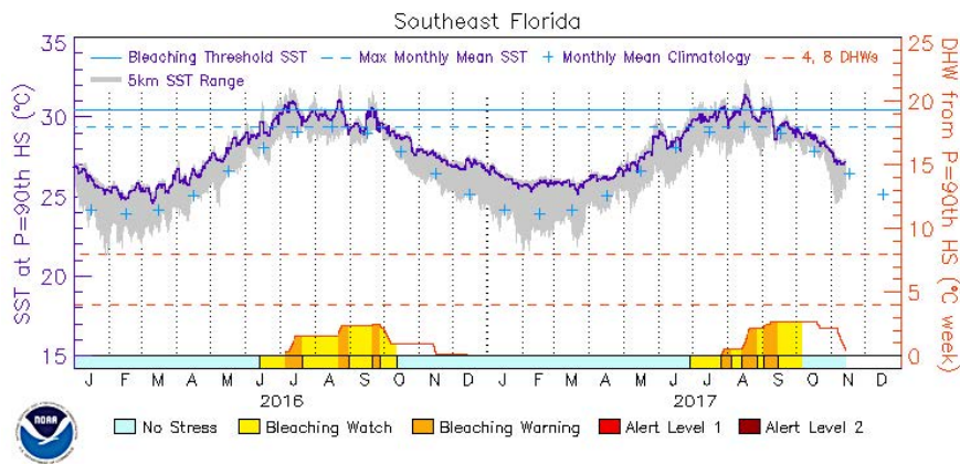
Figure 4. NOAA CRW Virtual Station Data; January 1, 2016 – November 13 2017. http://coralreefwatch.noaa.gov/vs/gauges/southeast_florida.php
