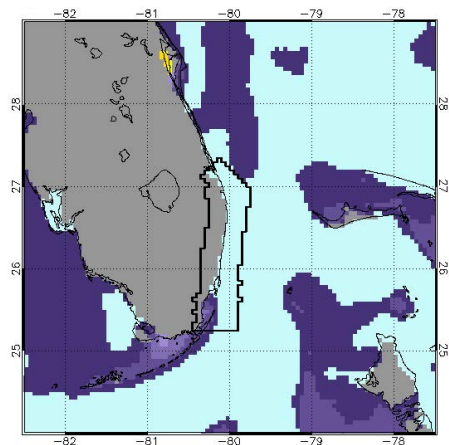
Figure 2 (left). NOAA CRW Hotspots for November 13, 2017. http://coralreefwatch.noaa.gov/satellite/bleaching5km/index.php
