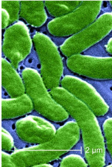
Coastal pathogens
